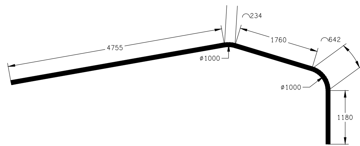
DETAIL C L3 LIGHT FITTING DIMENSIONS SCALE 1:50
